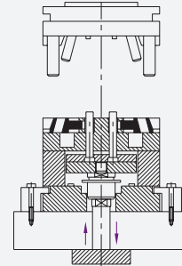
Mould Open-Coupler Engages & Pushes Forward
