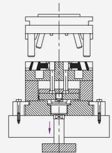
Coupler and Bars Pull Back the Ejector Plate
