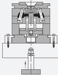
Mould Closed Material Injected
