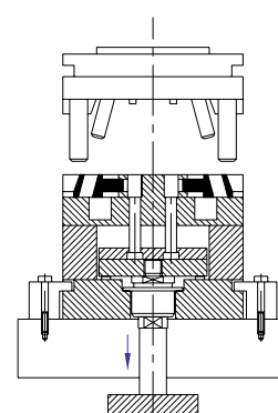
Coupler and Bars Pull Back the Ejector Plate
